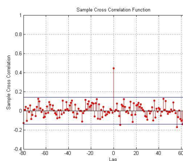
Crosscorr2&amp;3
