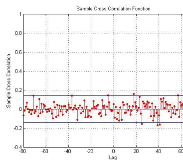
Crosscorr5&amp;6
