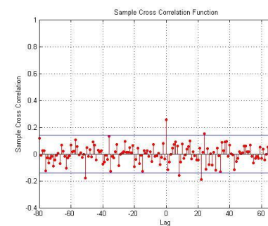
Crosscorr6&amp;7
