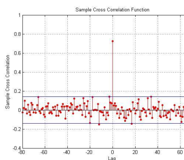
Crosscorr1&amp;2
