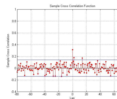
Crosscorr3&amp;4
